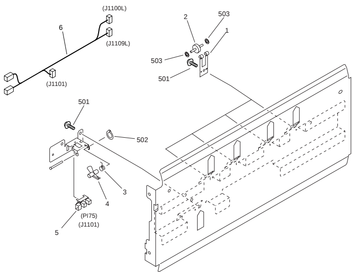
FIGURE Q32 RIGHT INNER GUIDE ASSEMBLY
